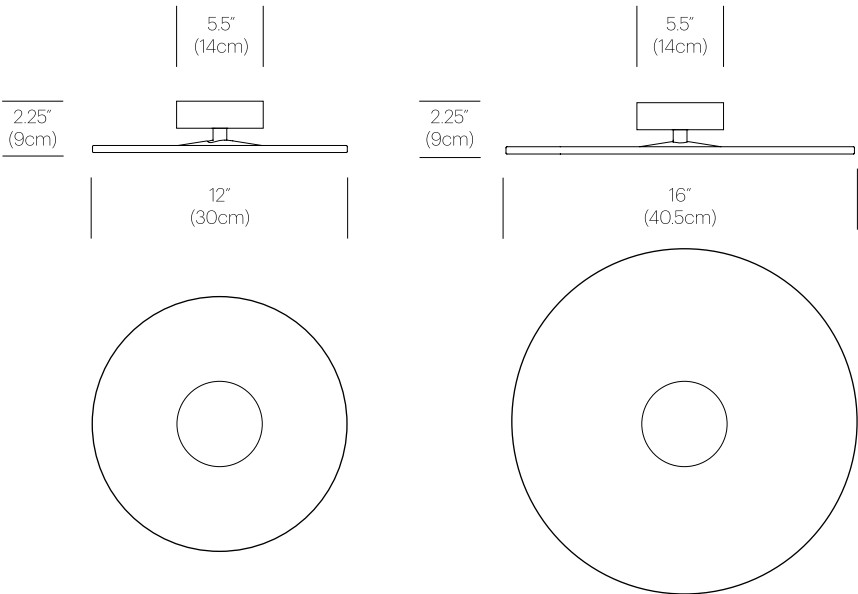
CIRCA FLUSH 12
